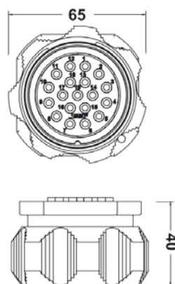
PANEL MALE Finger grip version
