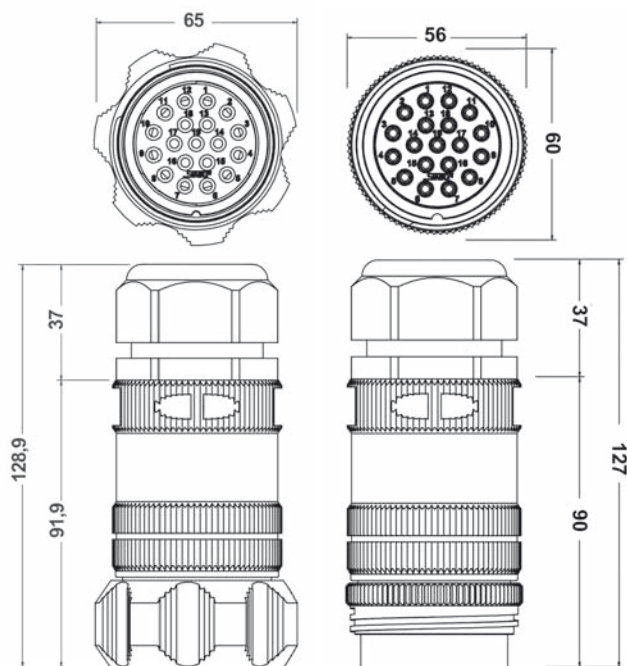
INLINE MALE (finger grip version) INLINE FEMALE (special version)
