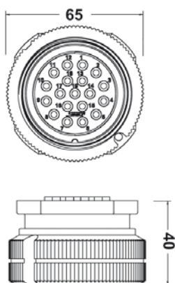
PANEL MALE Heavy duty version
