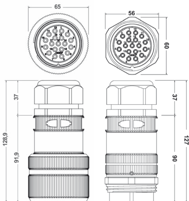
INLINE MALE and FEMALE Heavy duty version
